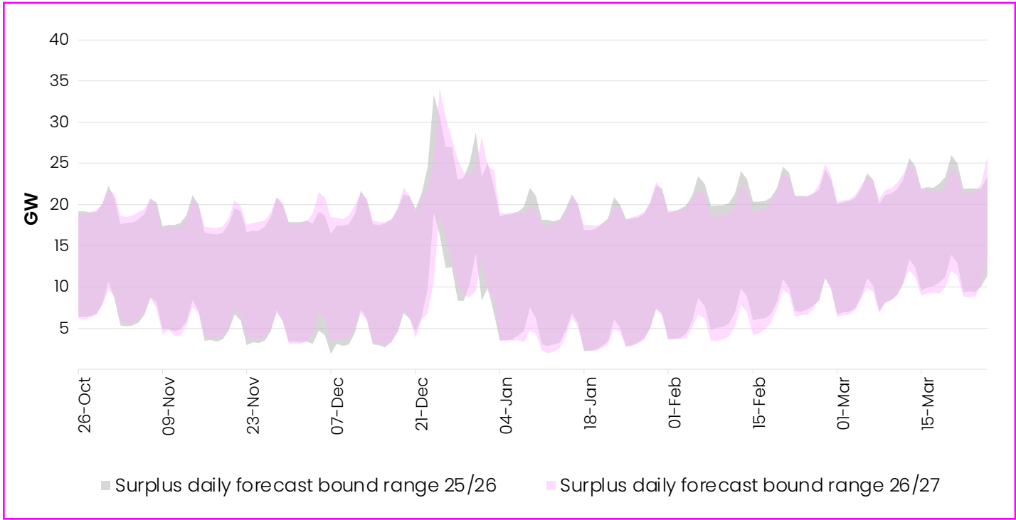
Figure 4: Daily forecast range of operational surplus for this winter (pink plume) compared with the forecast range in the Winter Outlook 2025/26 report (grey plume)
