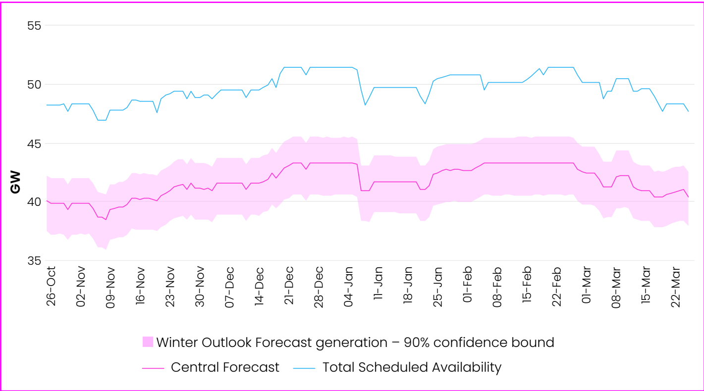
Figure 8: Planned generator availability for winter 2026/27, with the forecast range of de-rated generation availability and the central forecast of expected demand
