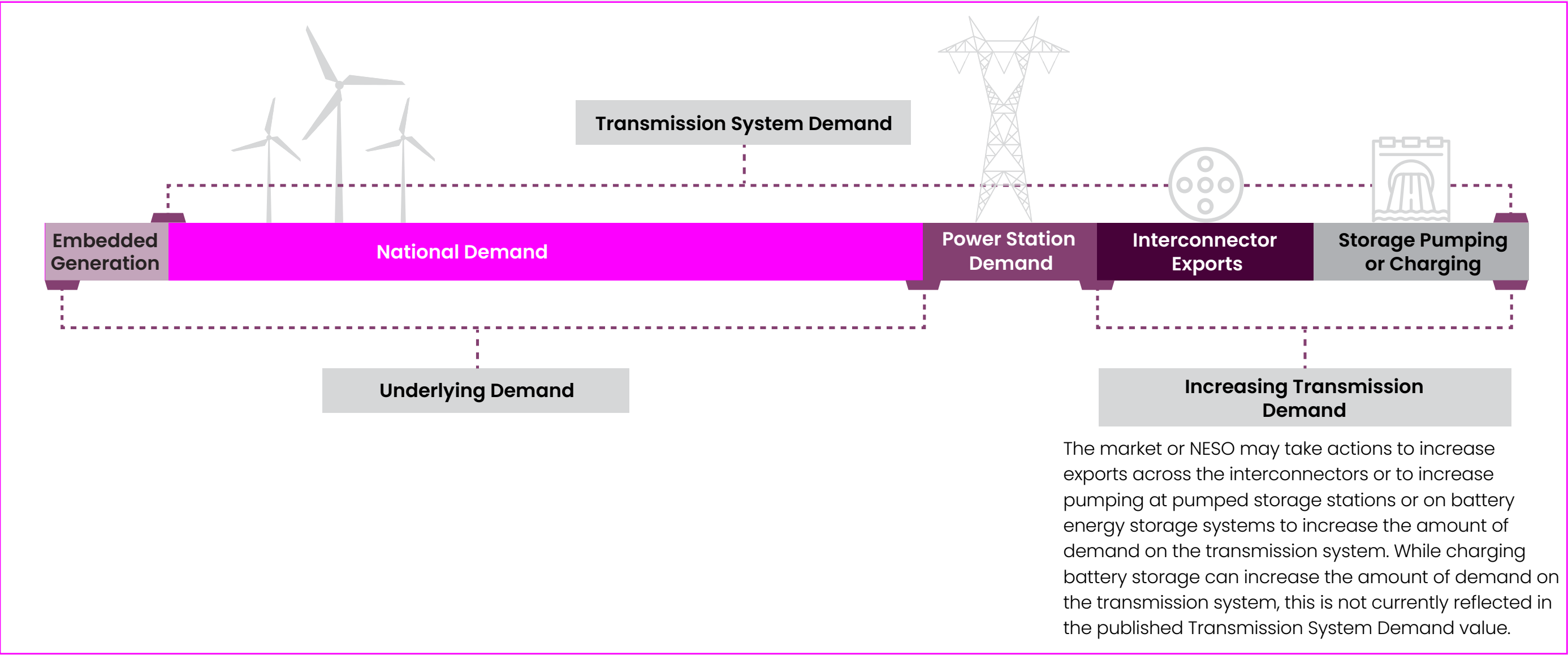
Figure 18: Relationship between some of the different types of demand (not to scale)
