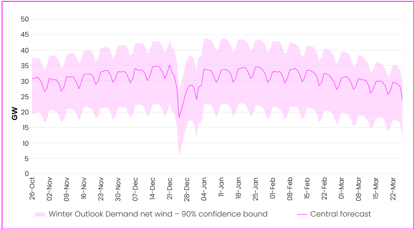
Figure 9: Forecast demand net wind for winter 2026/27
