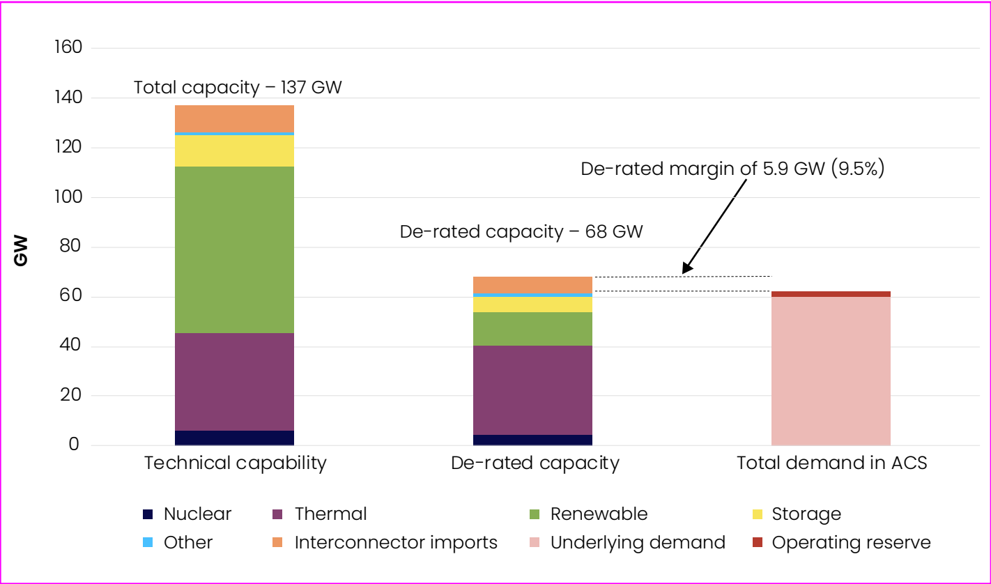
Figure 1: Total technical capacity of transmission- and distribution-connected supply and the resulting de-rated contribution during a period of system stress, shown against ACS peak demand
