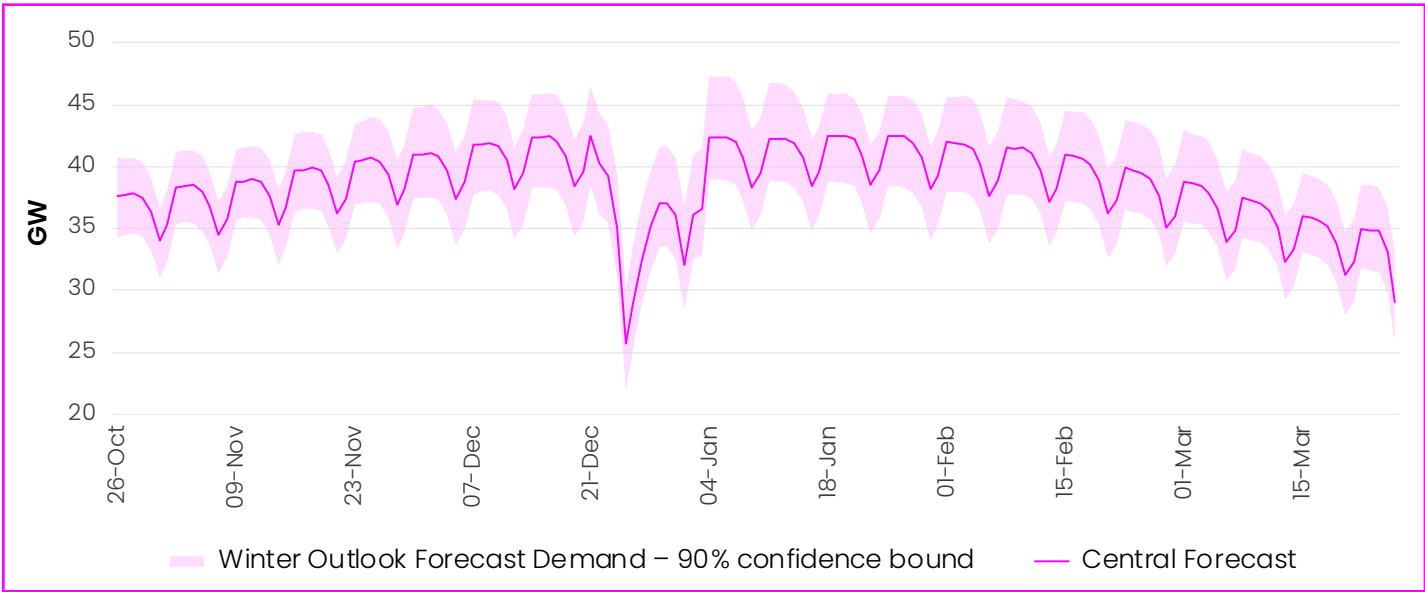
Figure 6: Forecast range of peak National Demand for winter 2026/27
