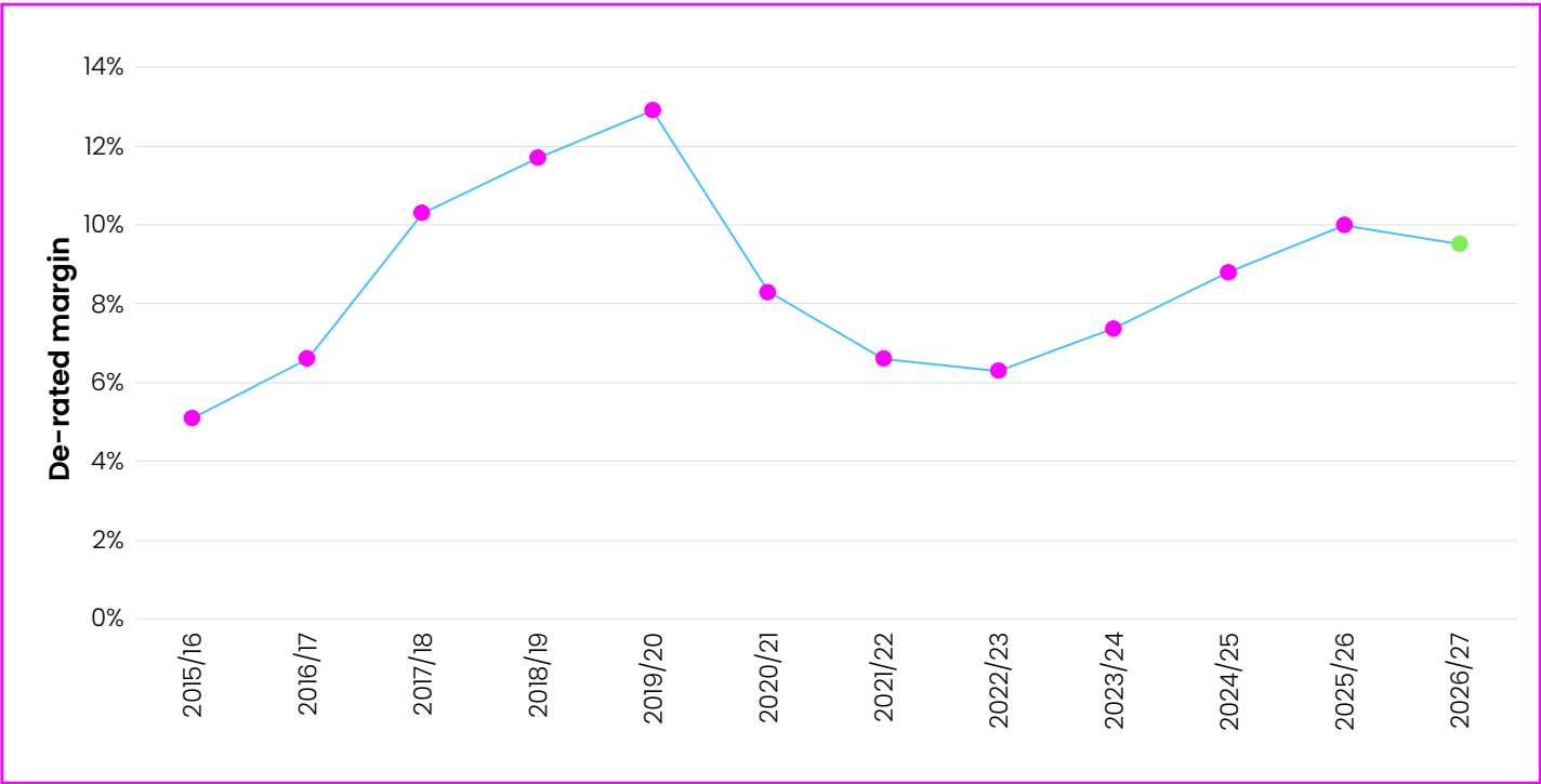
Figure 3: Historic de-rated margin forecasts made ahead of each winter in the Winter Outlook reports. The figure for 2026/27 is derived from our updated modelling approach and is therefore not directly comparable with figures from previous years.
