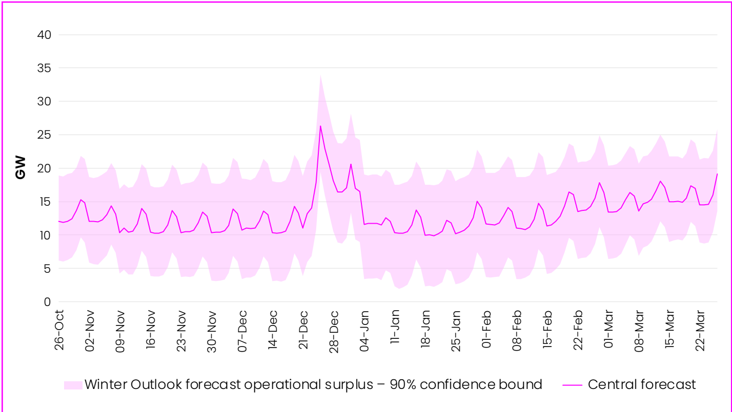
Figure 2: Range of outcomes for the daily operational surplus in our base case under different supply and demand conditions. This is the 90% confidence level and we therefore expect days when the operational surplus falls below the shaded range.
