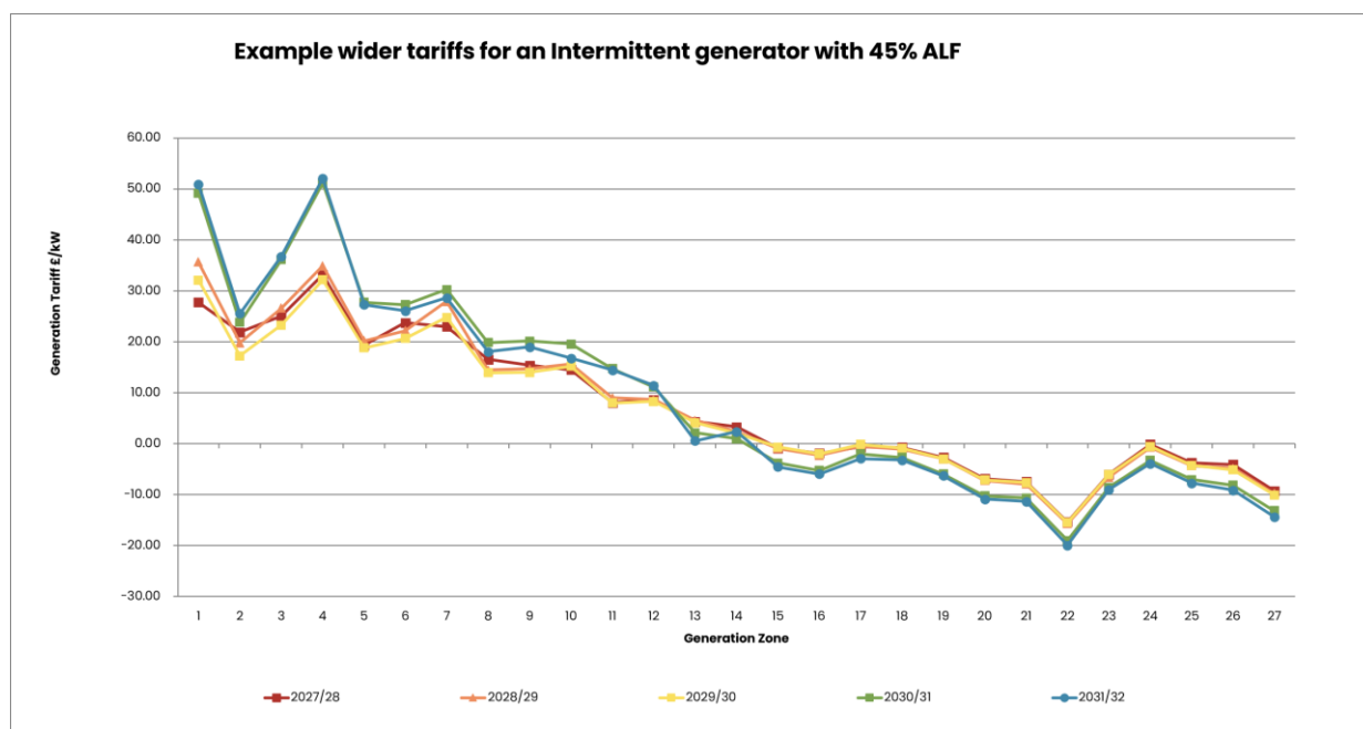
Figure 3 Example Wider tariffs for an Intermittent generator with an ALF of 45%
