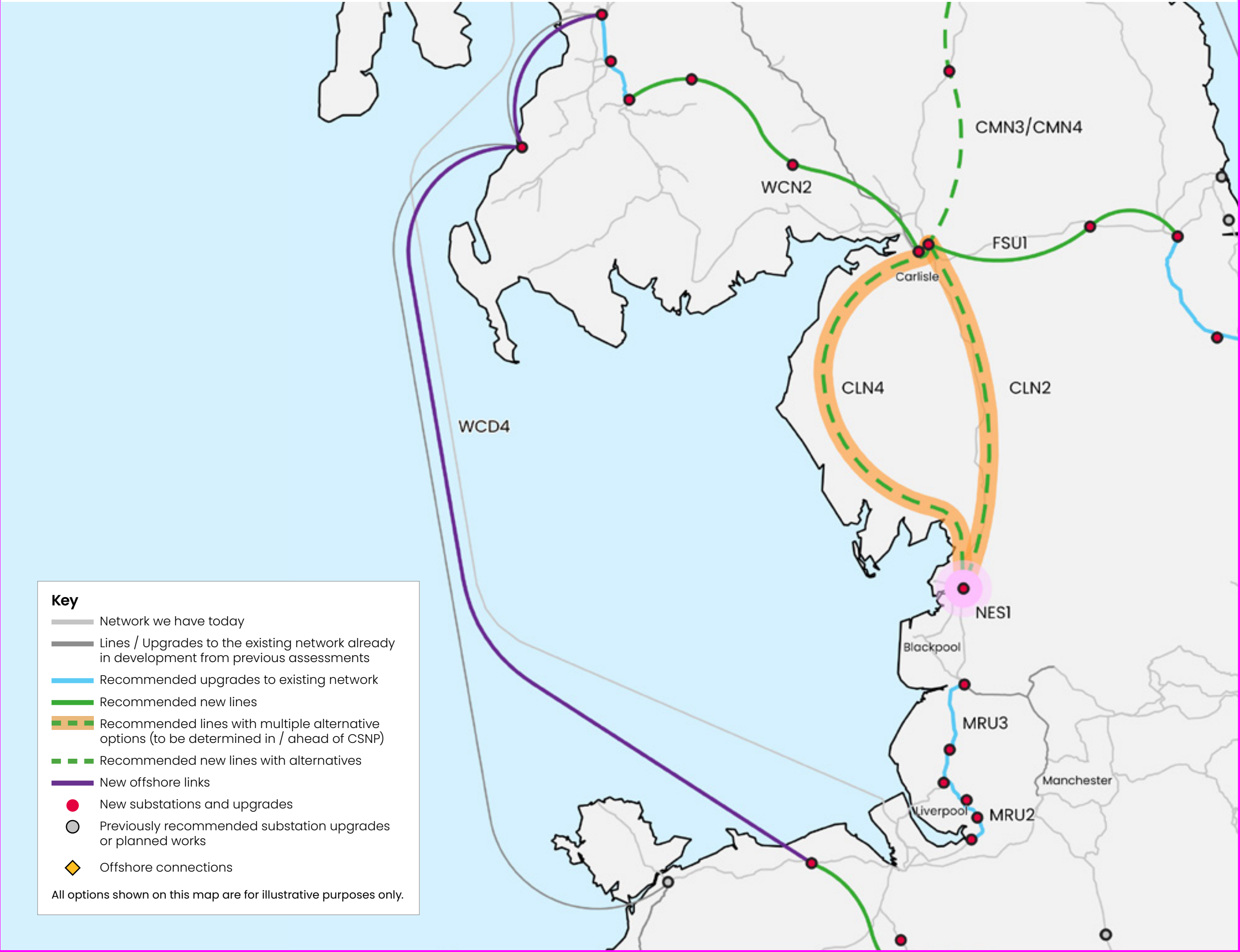
Figure 16: Map of the recommended network for North West
