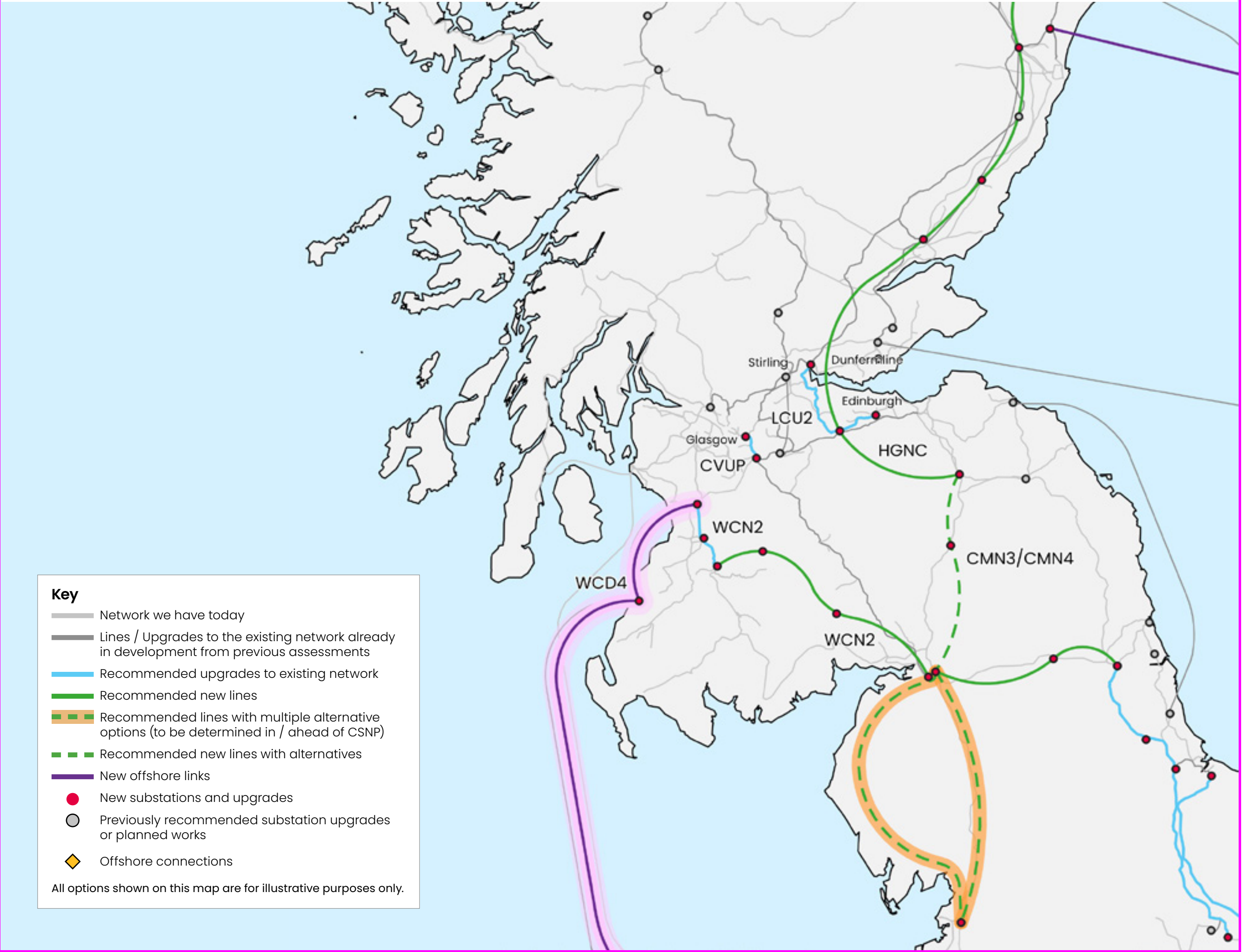
Figure 15: Map of the recommended network for Central and Southern Scotland
