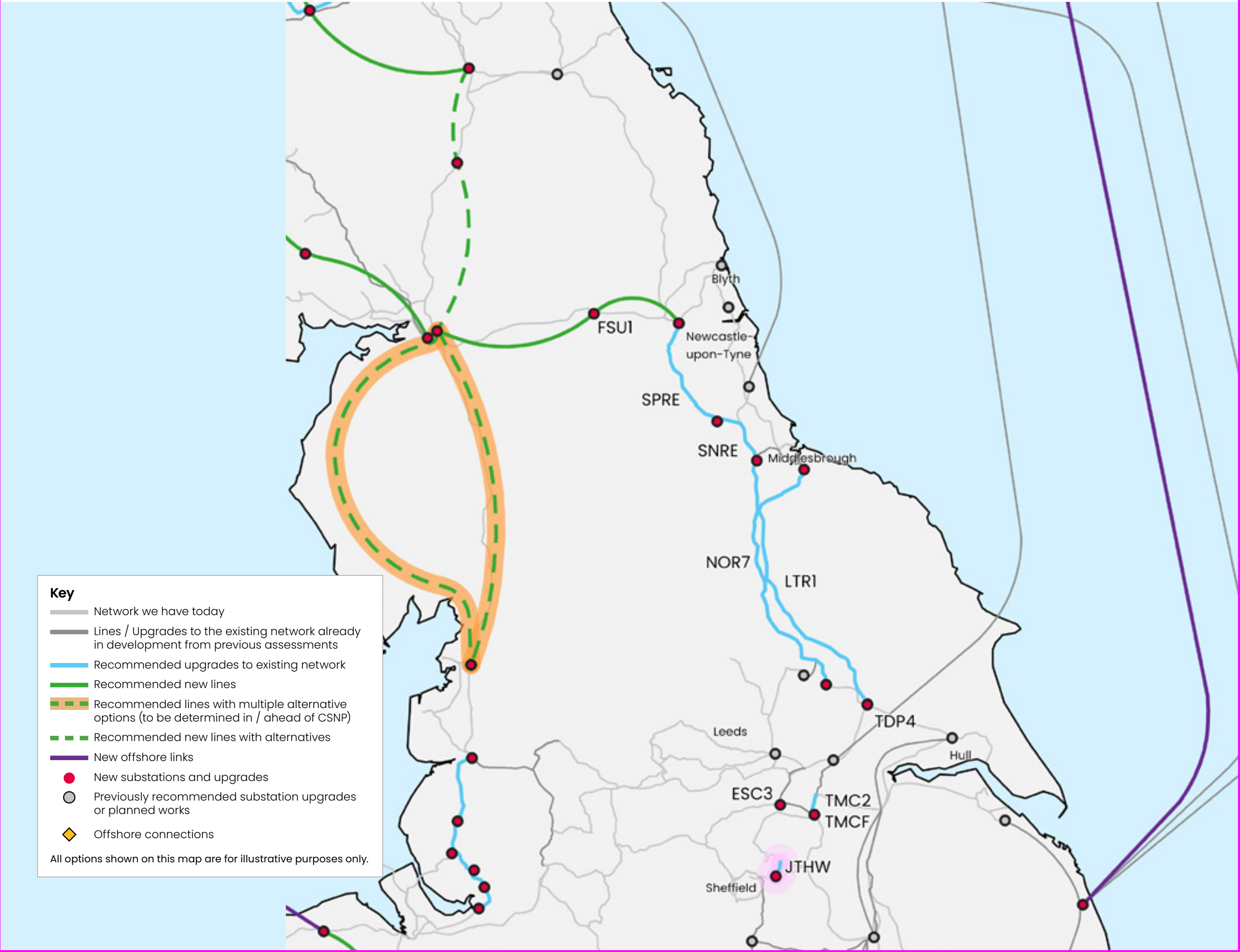
Figure 17: Map of the recommended network for North East and Yorkshire
