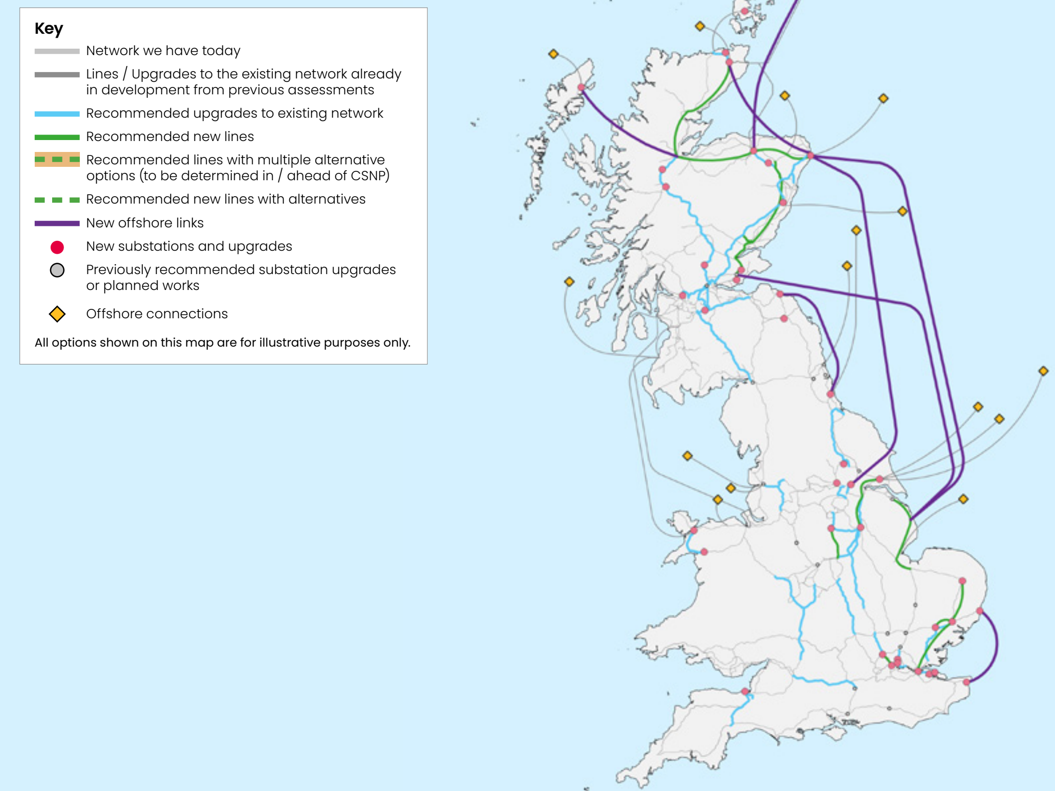
Figure 10: Map of the network for 2030, including options where we previously identified acceleration to 2030 would be beneficial
