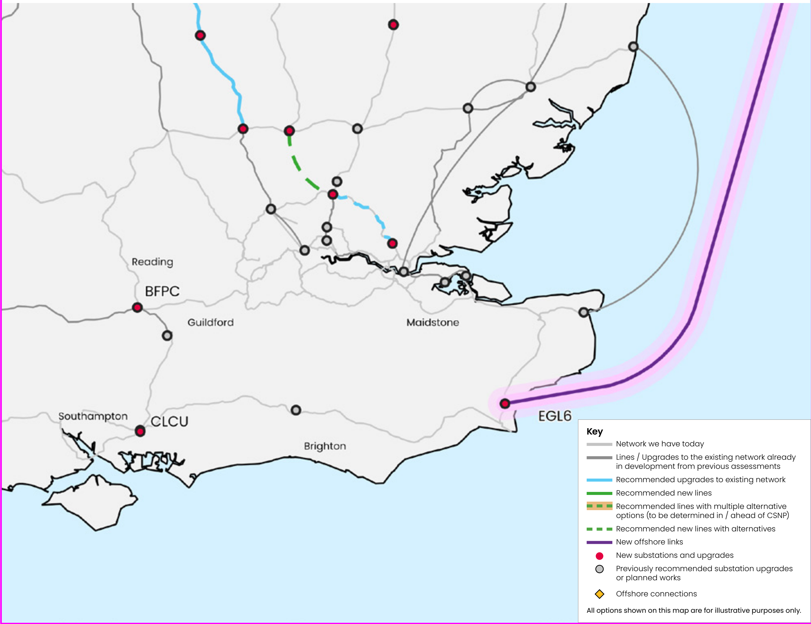
Figure 21: Map of the recommended network for South East
