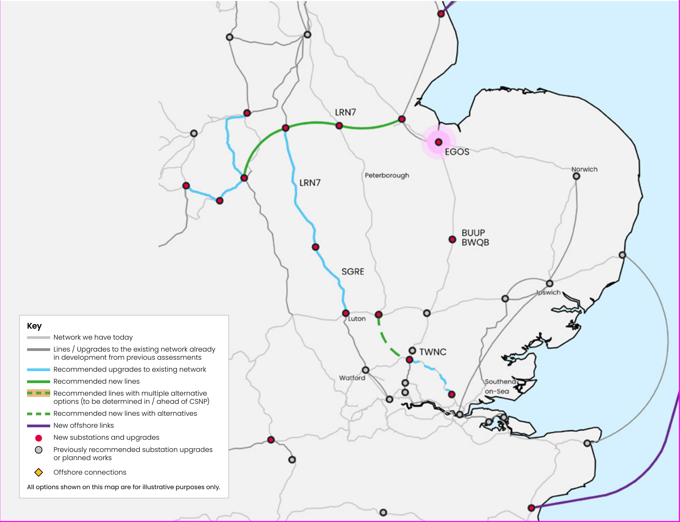
Figure 20: Map of the recommended network for central England and East of England
