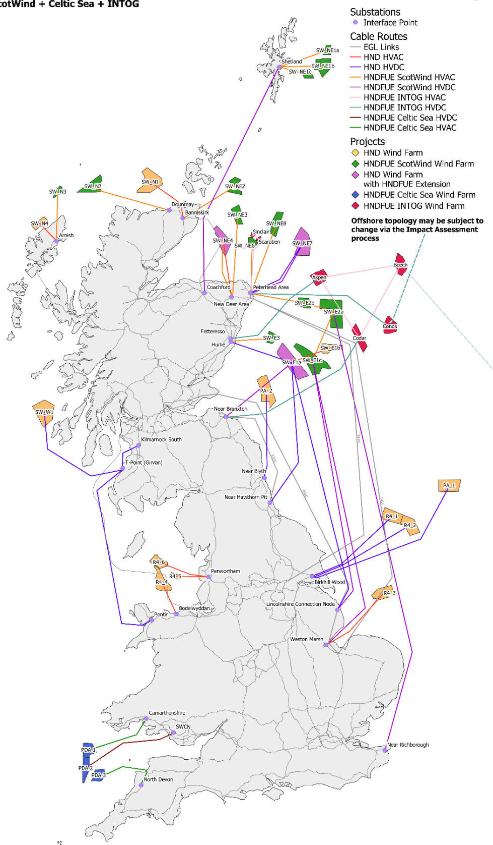
Figure 7: Schematic representation of complete HND and HNDFUE Recommended Designs (the Plan)
