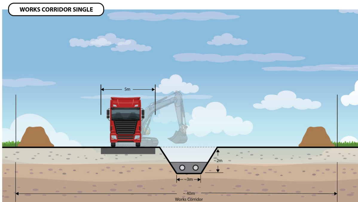
Figure 37: Example single trench working strip
