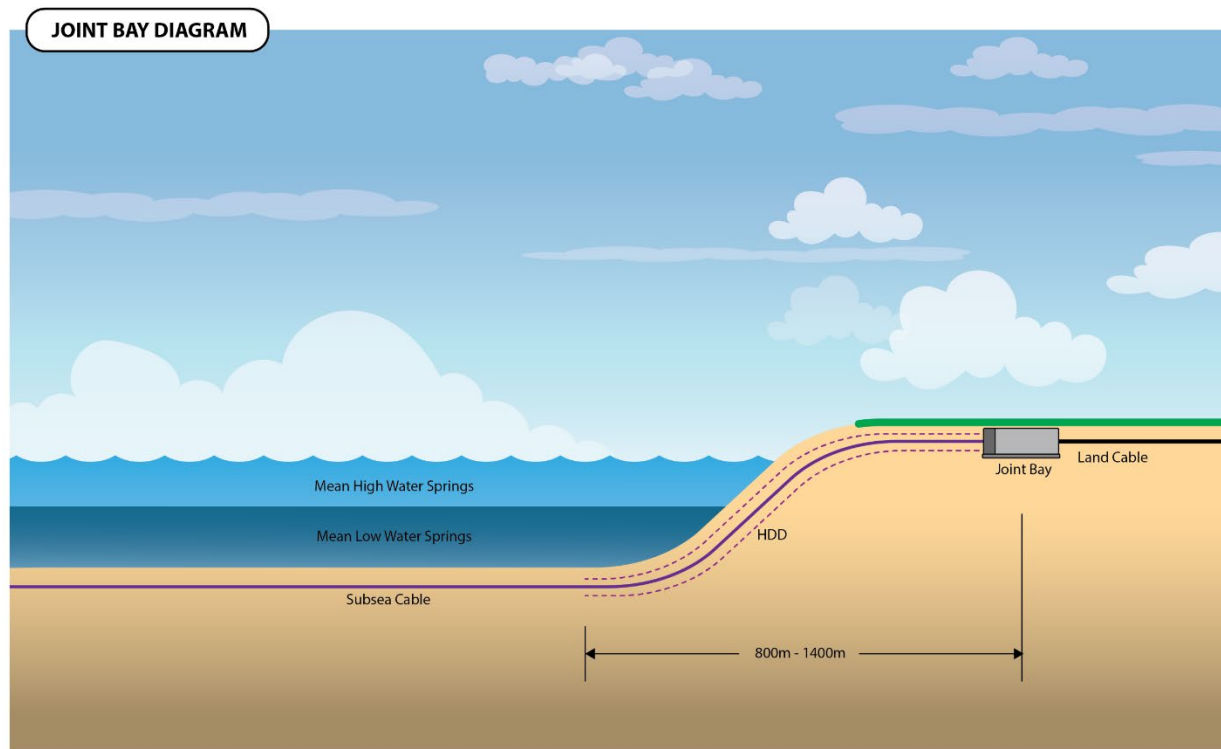
Figure 36: Landfall HDD
