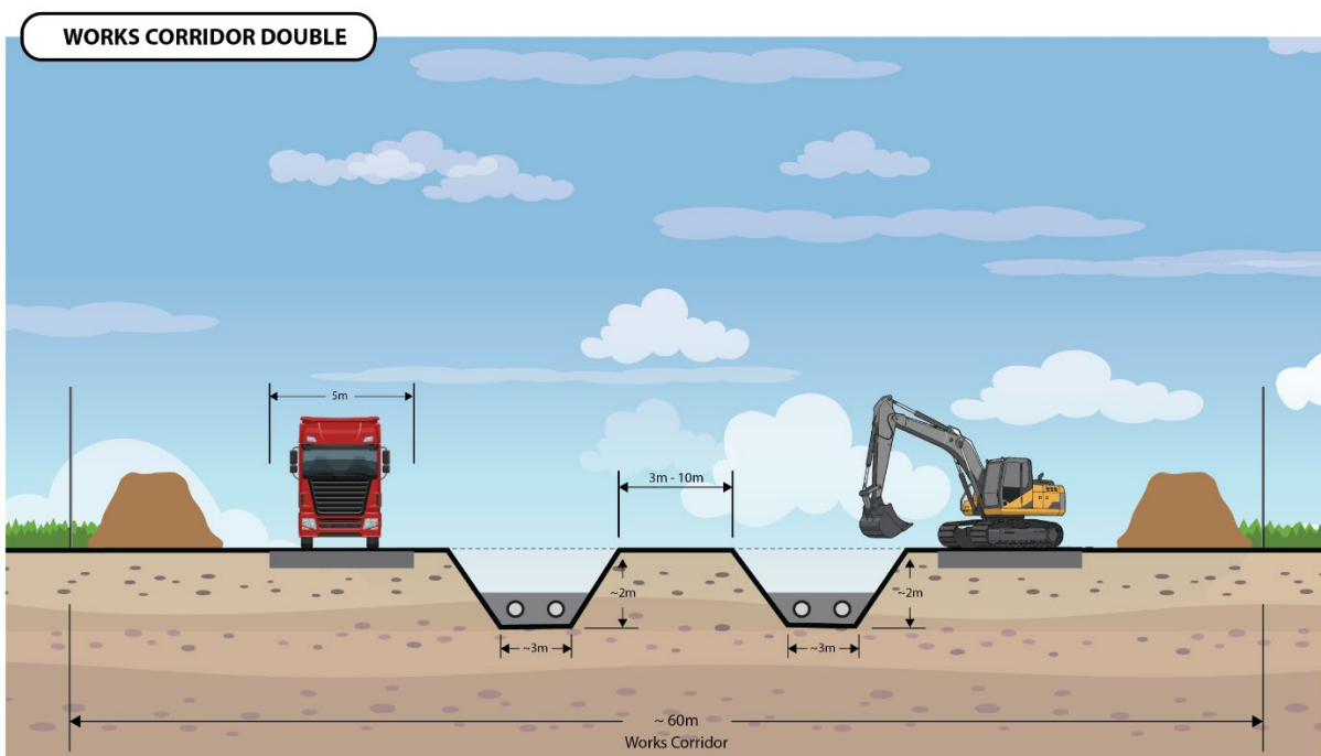
Figure 38: Example double trench working strip
