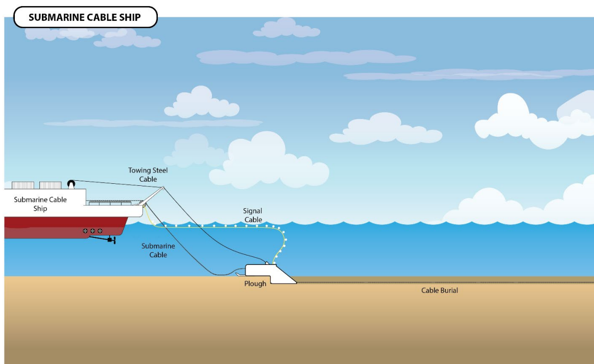
Figure 35: Typical submarine cable laying set-up
