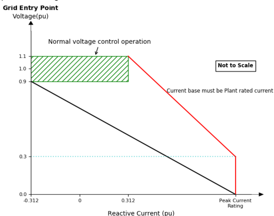
Figure 3: The reactive current to be supplied under a faulted condition
