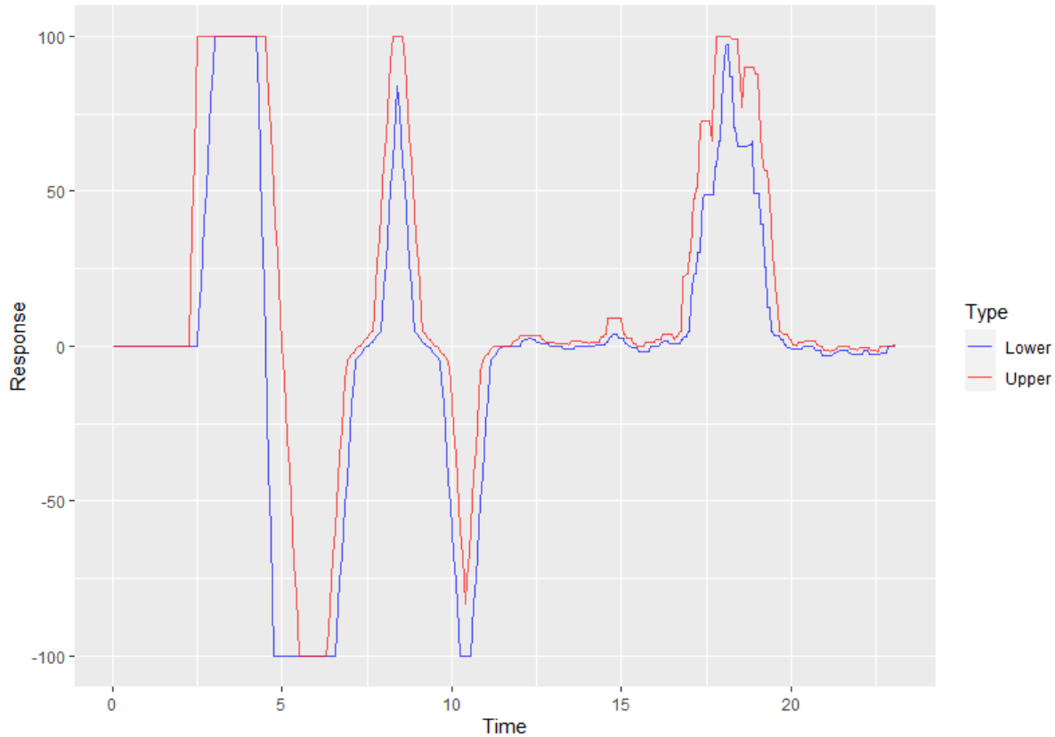
Figure 2: Example of symmetric performance bounds calculation using the frequency bounds from figure 1
