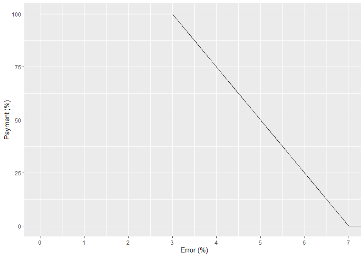
Figure 3: Payment adjustment (K factor) curve
