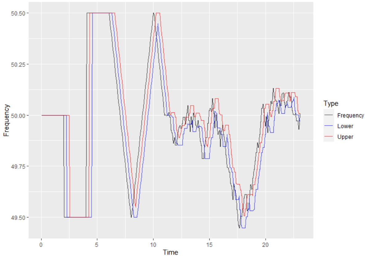
Figure 1: Example of frequency bounds calculation
