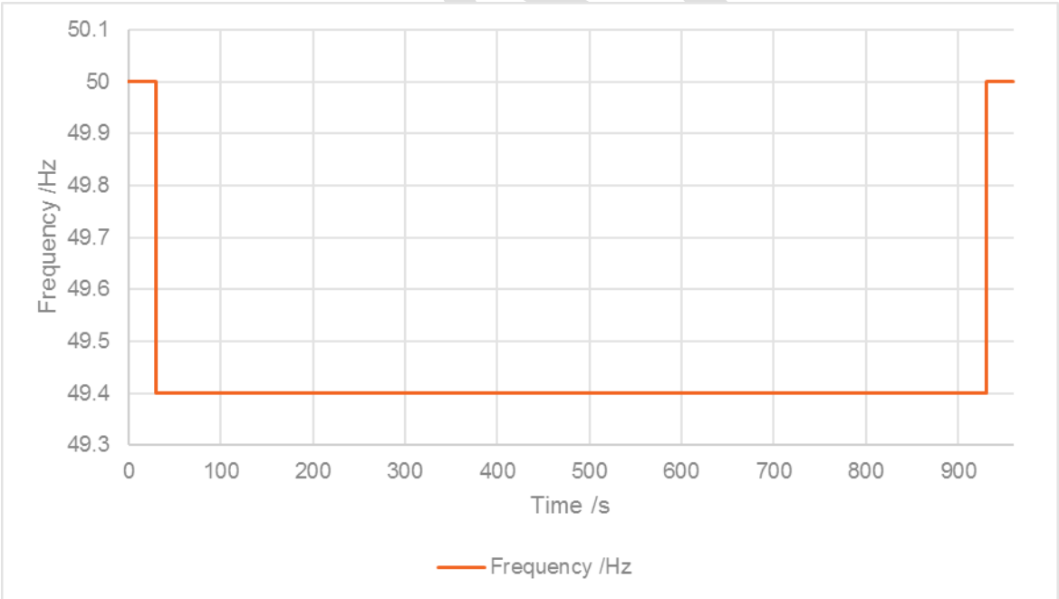
Figure 10 Test 3.2 Injection Profile
