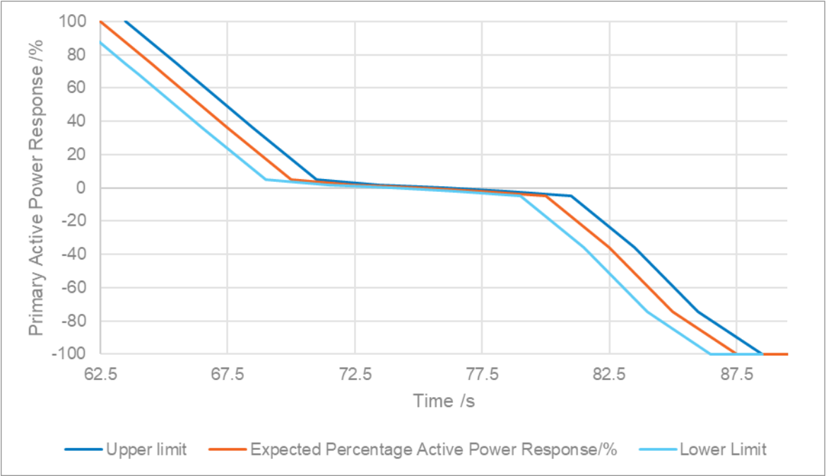
Figure 7 - Test 2.1b Tolerance - sample
