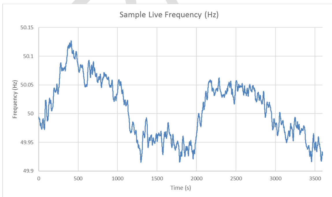
Figure 11 - Sample System Frequency
