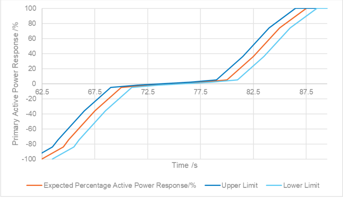
Figure 8 - Test 2.2b Tolerance - sample
