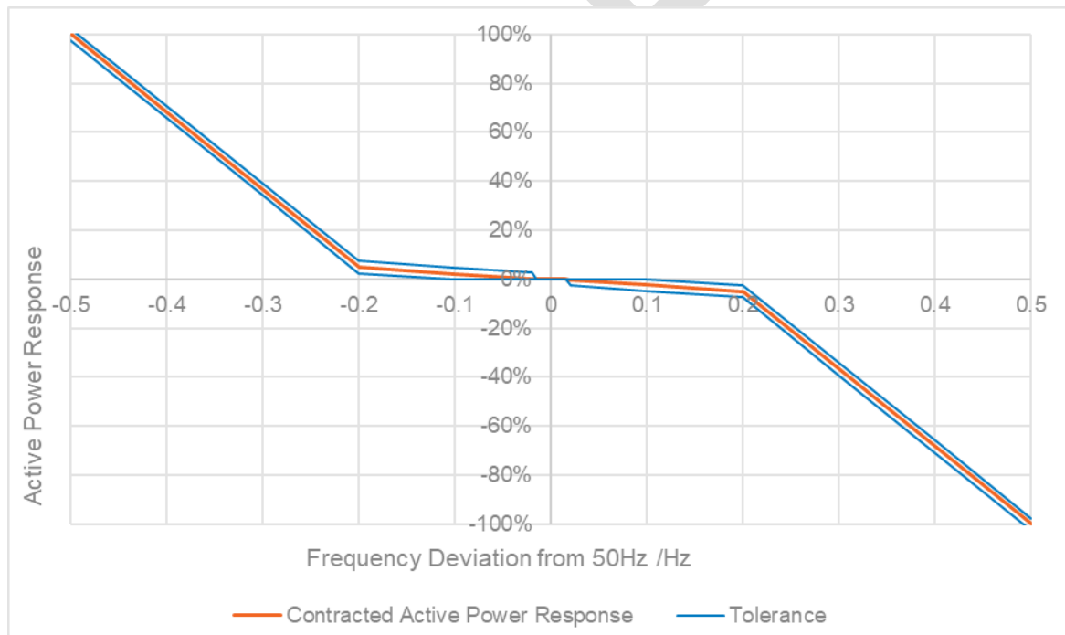
Figure 3 Graphical representation of tolerance bands for the expected response at different frequencies – sample chart only
